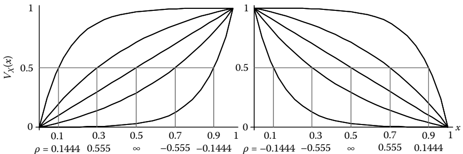
Figure 3.5: Families of exponential value functions.
