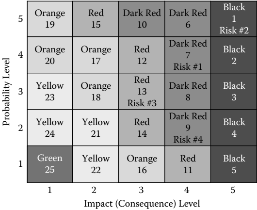
Figure 4.10: Risk events #1 through #4: combined view.
