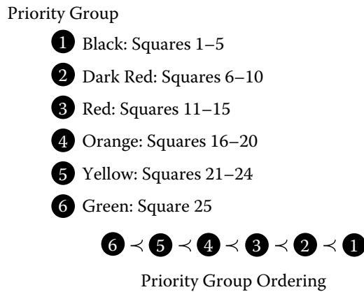
Figure 4.9: Priority group ordering in Figure 4.8.
