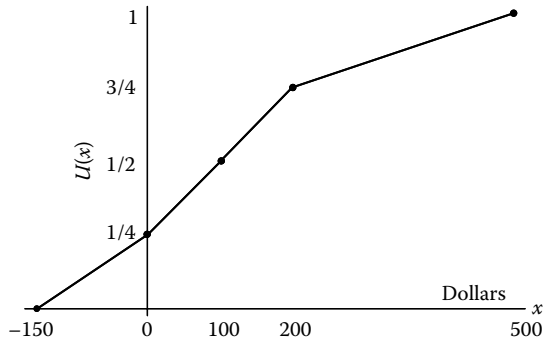
Figure 3.23: A 5-point defined utility function.
