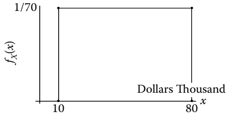
Figure 3.22: A uniform probability density function.
