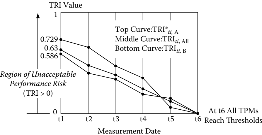
Figure 4.39: Illustrative TPM risk index time-history trend.
