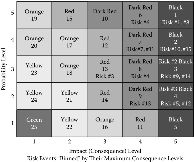
Figure 4.10C: An ordinal risk matrix mapping of Table 4.8A risks.
