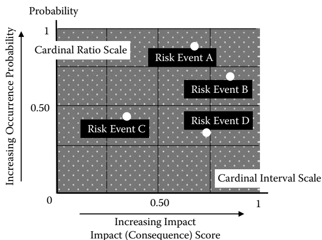
Figure 4.11: A risk matrix defined by cardinal scales.
