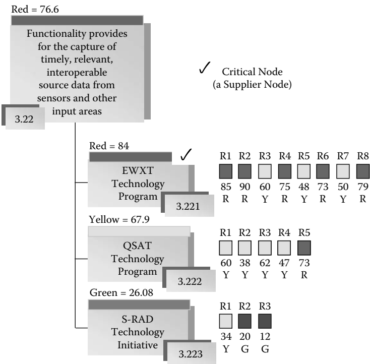
Figure 4.57: Risk measure derived for functionality 3.22.
