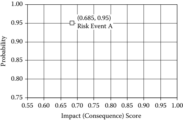
Figure 4.15: Case Discussion 4.1: a plot of risk event A .
