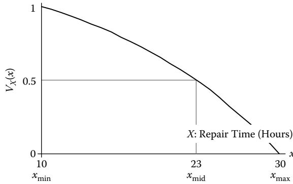
Figure 3.6: An exponential value function for Repair Time.
