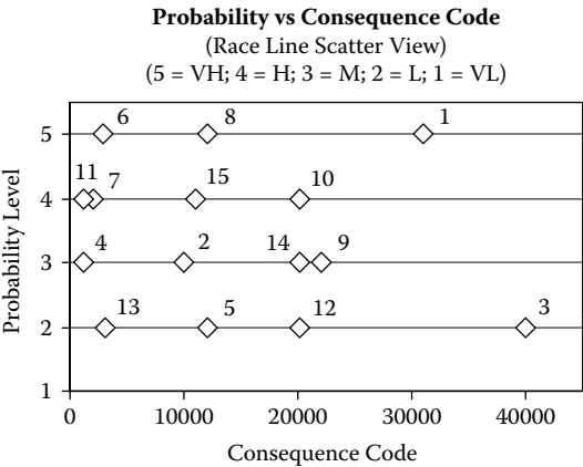
Figure 4.10B: Probability level vs. consequence code.
