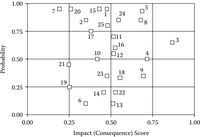
Figure 4.16: A scatter plot of 25 risk events.
