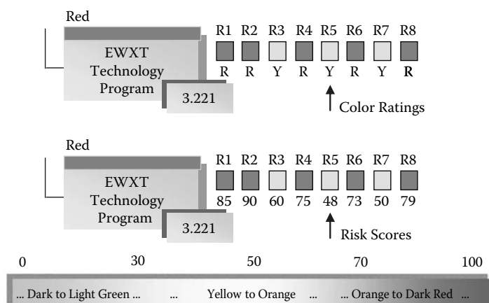
Figure 4.52: Example risk scores for EWXT program risks. (R = Red, Y = Yellow)
