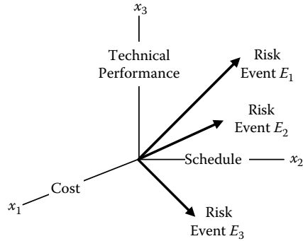
Figure 3.26: Typical risk impact dimensions.
