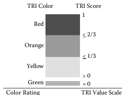
Figure 4.43: A possible TRI color scheme.
